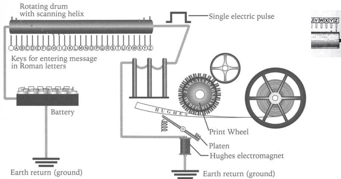
The Hughes telegraph system showing the keys and scanning rotating helix of the transmitter. Pressing any key resulted in the transmission of a single electrical pulse which activated a Hughes relay in the (synchronized) receiving instrument, causing the rapid release of the platen and the printing of the letter on a moving paper tape.
